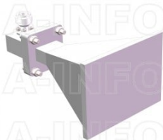
LB-90-15-C-NFSPO Standard Gain Horn Antenna 8.2-12.4GHz 15dB Gain N Type Female
